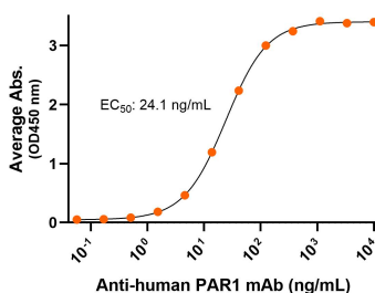
Anti-human PAR1 Monoclonal Antibody, ELISA 0.2µg of PAR1 ECD1 per well
